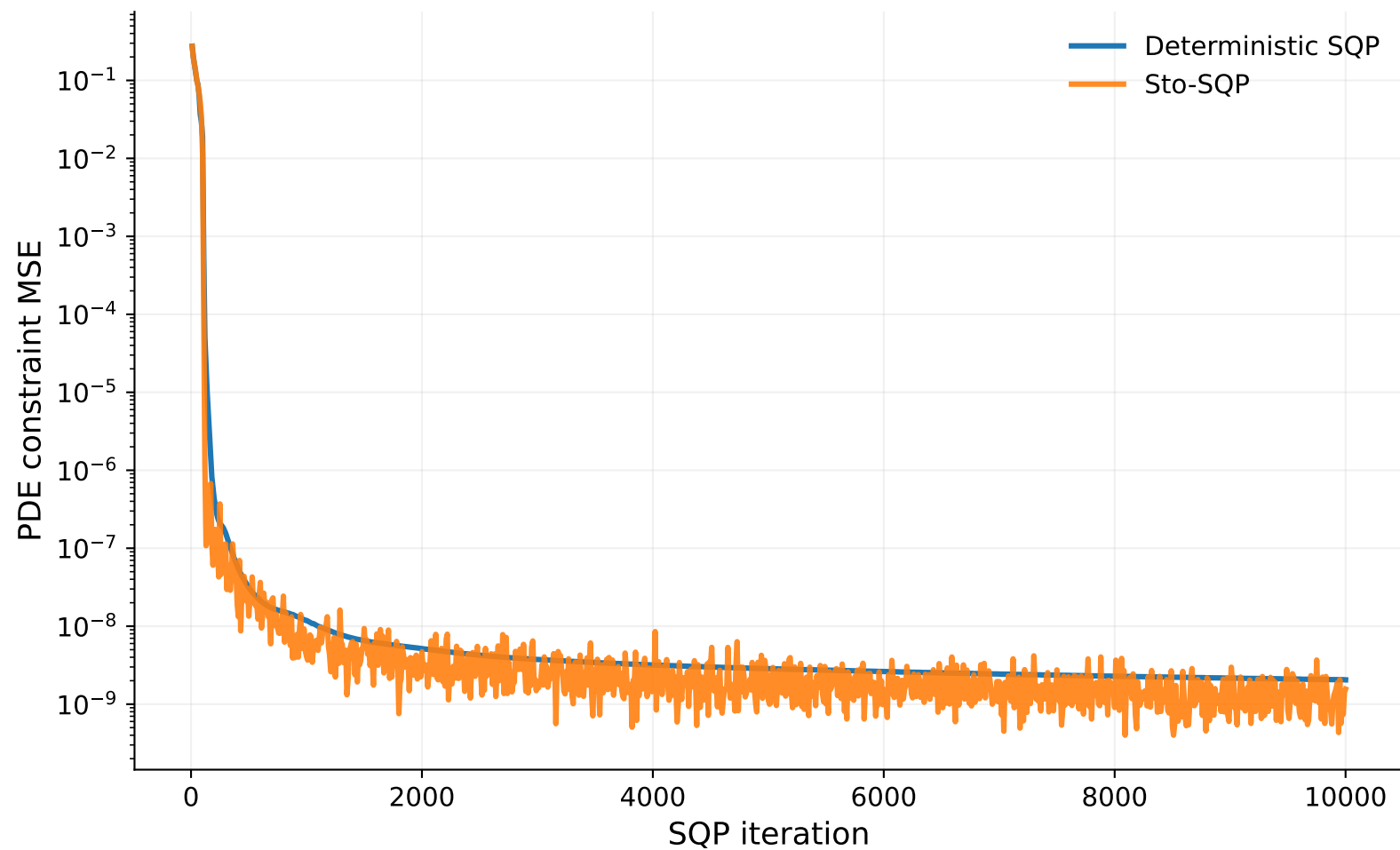
Burgers equation: PDE constraint MSE — full trajectory
