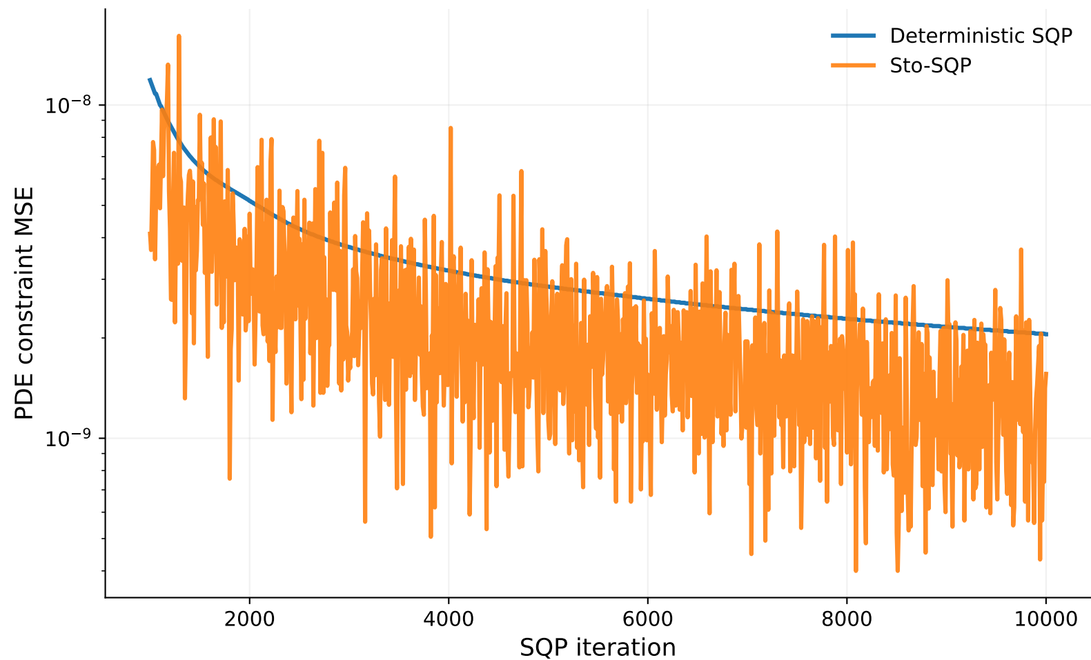
Burgers equation: PDE constraint MSE — zoom: iter \geq 1000
